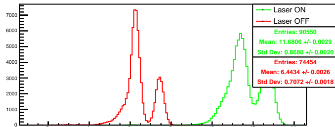
Run 4537 quartetwise, negH0: Beam ON
