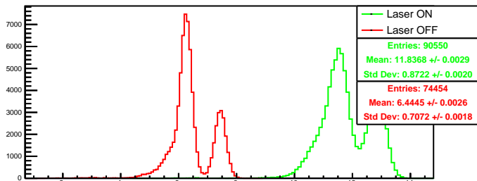
Run 4537 quartetwise, posH0: Beam ON
