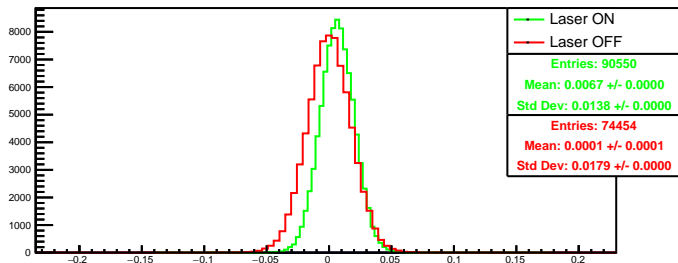
Run 4537 quartetwise, asym0: Beam ON
