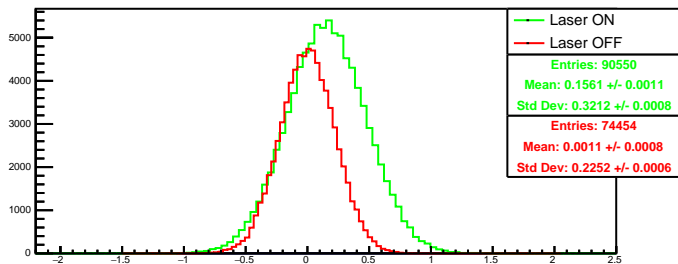
Run 4537 quartetwise, diff0: Beam ON
