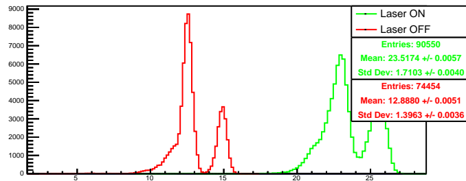
Run 4537 quartetwise, summ0: Beam ON
