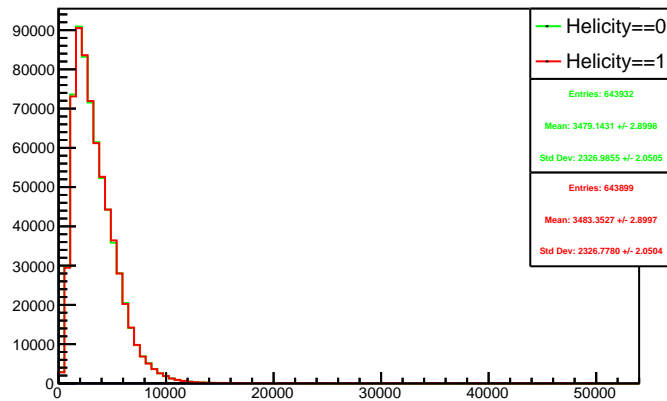
Run 4538 triggerwise, sums: Beam ON, Laser OFF
