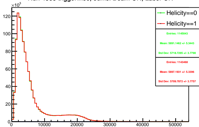
Run 4538 triggerwise, sums: Beam ON, Laser ON
