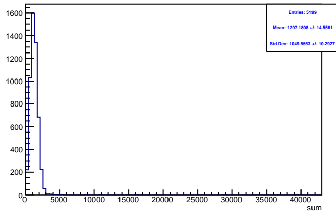
Run 4538 triggerwise, sums: Beam ON, Laser OFF
