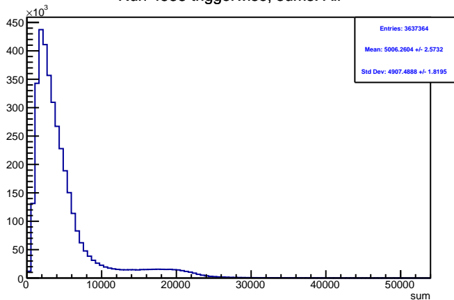
Run 4538 triggerwise, sums: All
