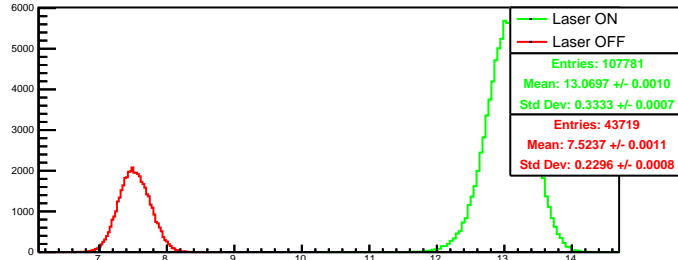
Run 4540 quartetwise, negH0: Beam ON
