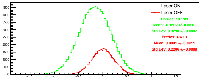
Run 4540 quartetwise, diff0: Beam ON
