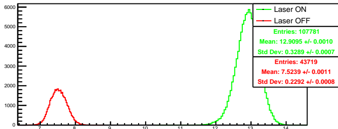
Run 4540 quartetwise, posH0: Beam ON
