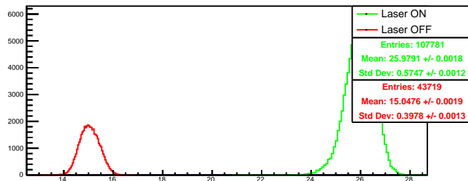
Run 4540 quartetwise, summ0: Beam ON
