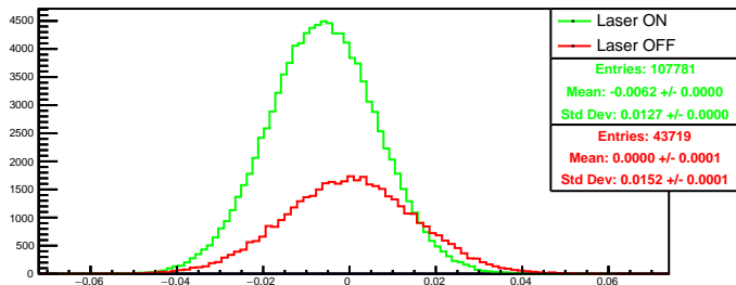
Run 4540 quartetwise, asym0: Beam ON
