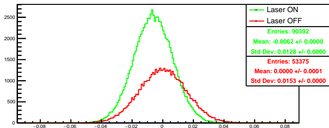
Run 4541 quartetwise, asym0: Beam ON
