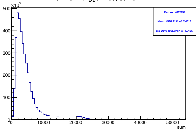
Run 4541 triggerwise, sums: All
