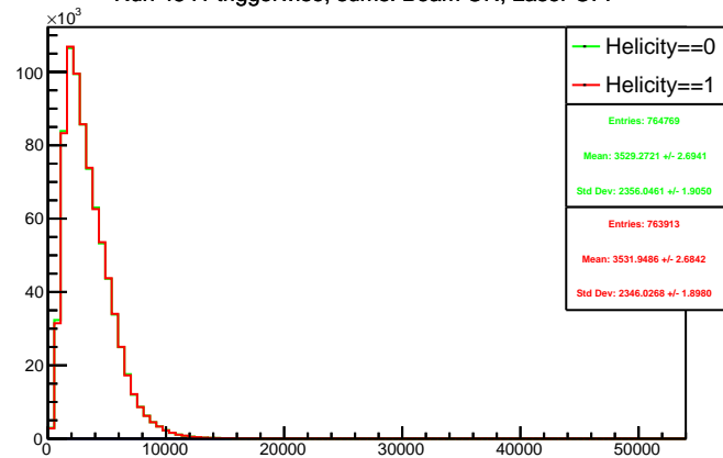
Run 4541 triggerwise, sums: Beam ON, Laser OFF
