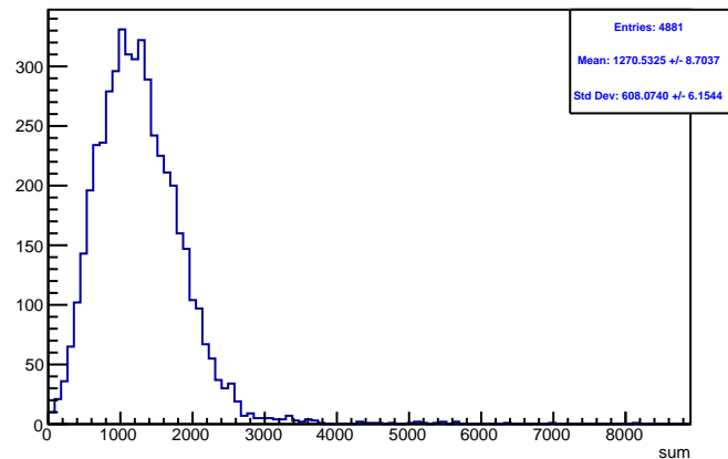
Run 4541 triggerwise, sums: Beam ON, Laser OFF
