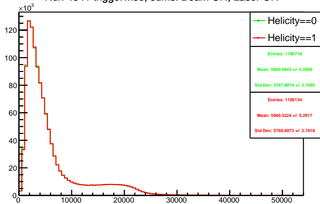
Run 4541 triggerwise, sums: Beam ON, Laser ON
