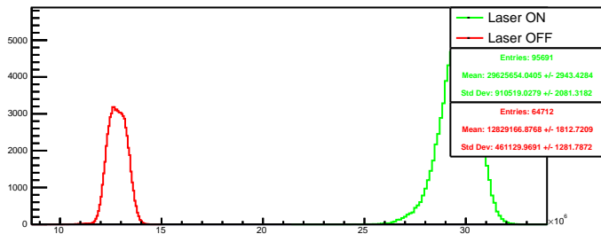
Run 4542 quartetwise, posH4: Beam ON
