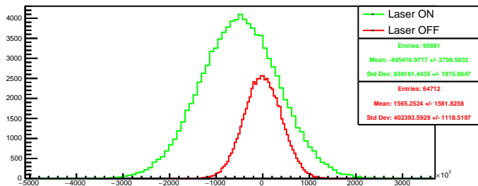
Run 4542 quartetwise, diff4: Beam ON
