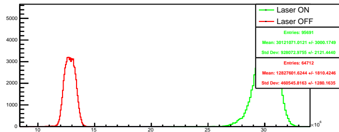
Run 4542 quartetwise, negH4: Beam ON
