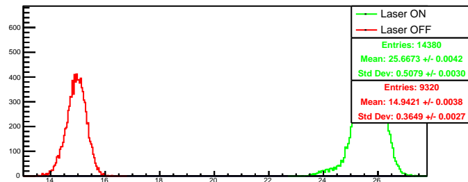
Run 4546 quartetwise, summ0: Beam ON
