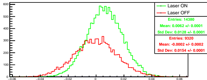
Run 4546 quartetwise, asym0: Beam ON
