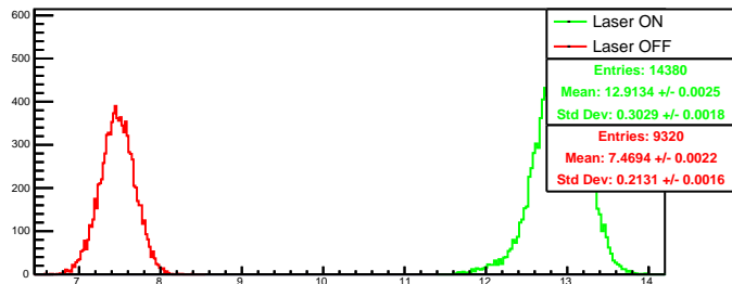
Run 4546 quartetwise, posH0: Beam ON
