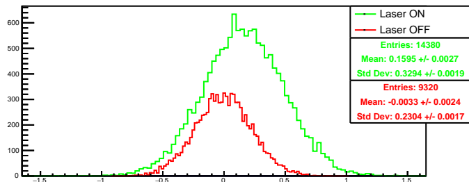
Run 4546 quartetwise, diff0: Beam ON
