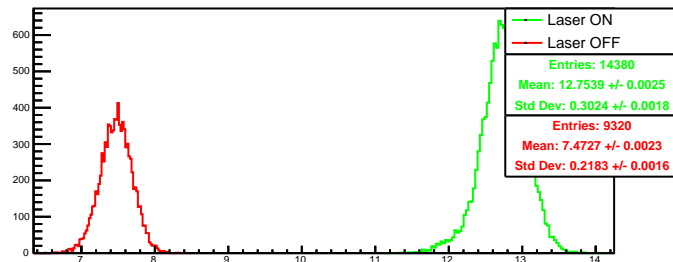
Run 4546 quartetwise, negH0: Beam ON
