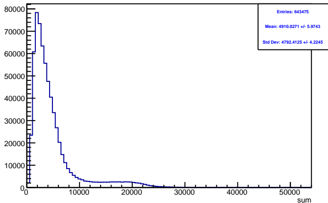
Run 4546 triggerwise, sums: Beam ON, Laser ON
