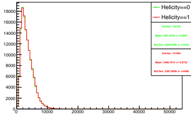
Run 4546 triggerwise, sums: Beam ON, Laser OFF
