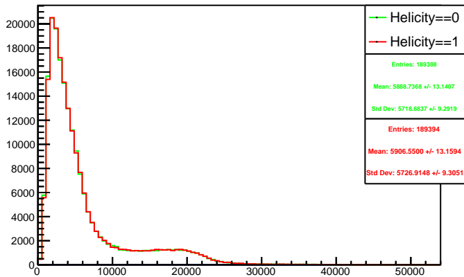
Run 4546 triggerwise, sums: Beam ON, Laser ON
