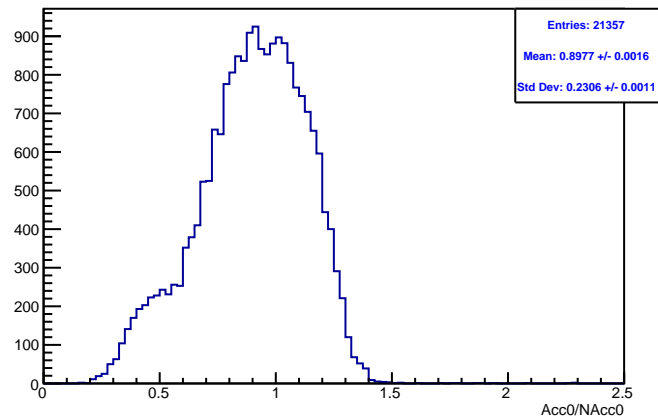
Run 4548 mpwise, acc0: Beam ON, Laser OFF
