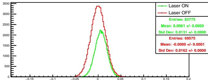
Run 4548 quartetwise, asym0: Beam ON
