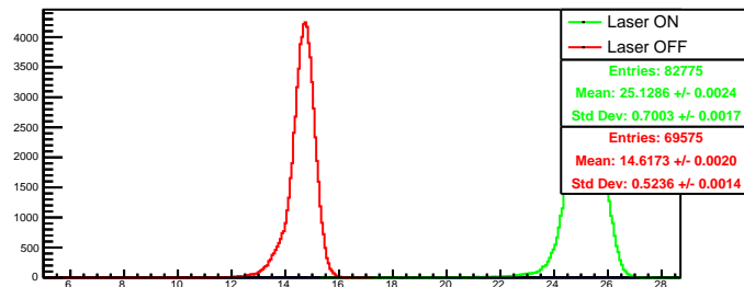
Run 4548 quartetwise, summ0: Beam ON
