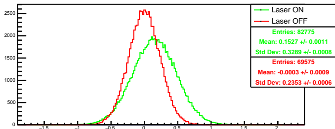
Run 4548 quartetwise, diff0: Beam ON
