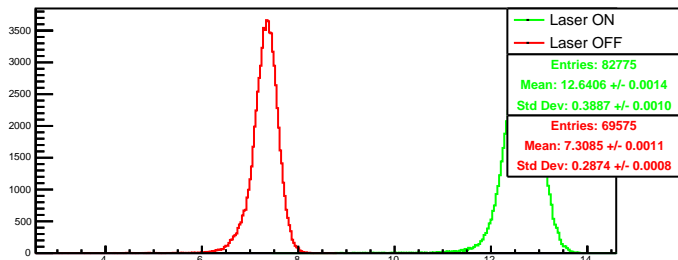
Run 4548 quartetwise, posH0: Beam ON
