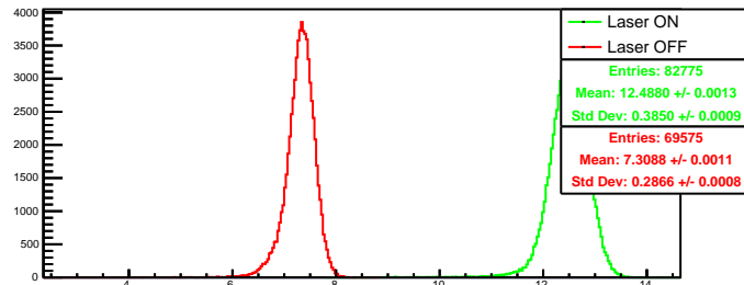
Run 4548 quartetwise, negH0: Beam ON
