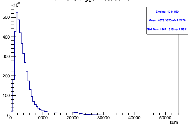
Run 4548 triggerwise, sums: All
