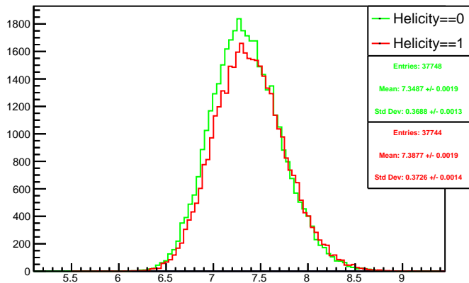
Run 4549 mpwise, acc0: Beam ON, Laser OFF
