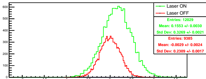
Run 4549 quartetwise, diff0: Beam ON
