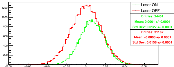
Run 4550 quartetwise, asym0: Beam ON
