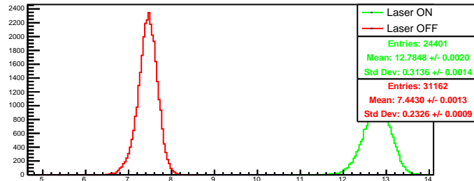
Run 4550 quartetwise, negH0: Beam ON
