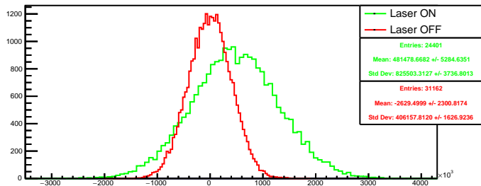
Run 4550 quartetwise, diff4: Beam ON
