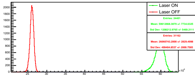
Run 4550 quartetwise, summ4: Beam ON
