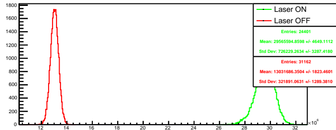
Run 4550 quartetwise, negH4: Beam ON
