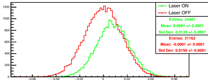
Run 4550 quartetwise, asym4: Beam ON
