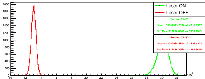
Run 4550 quartetwise, posH4: Beam ON
