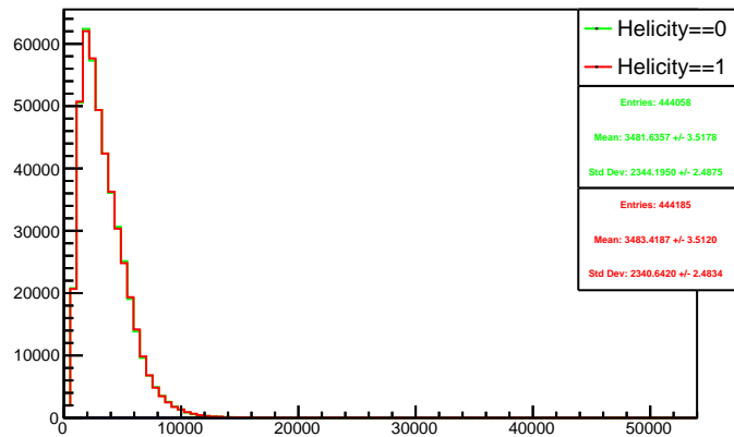
Run 4550 triggerwise, sums: Beam ON, Laser OFF
