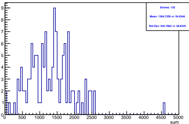
Run 4550 triggerwise, sums: Beam ON, Laser OFF
