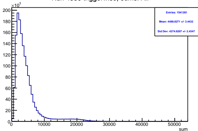
Run 4550 triggerwise, sums: All
