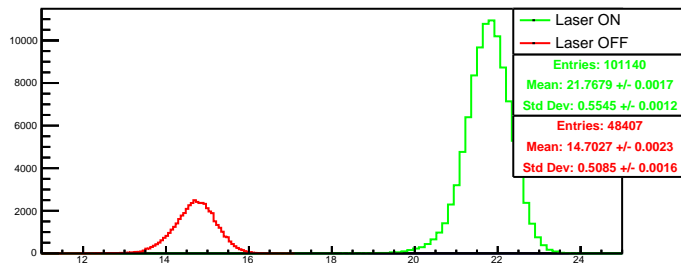
Run 4555 quartetwise, summ0: Beam ON
