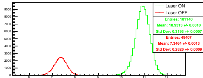
Run 4555 quartetwise, negH0: Beam ON
