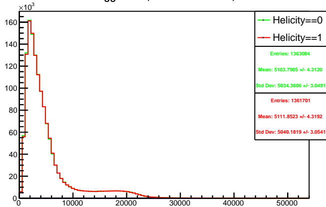
Run 4555 triggerwise, sums: Beam ON, Laser ON
