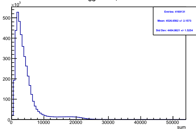
Run 4555 triggerwise, sums: All
