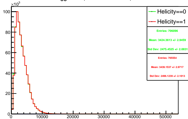
Run 4555 triggerwise, sums: Beam ON, Laser OFF
