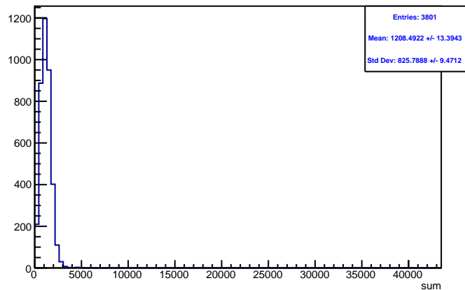
Run 4555 triggerwise, sums: Beam ON, Laser OFF
