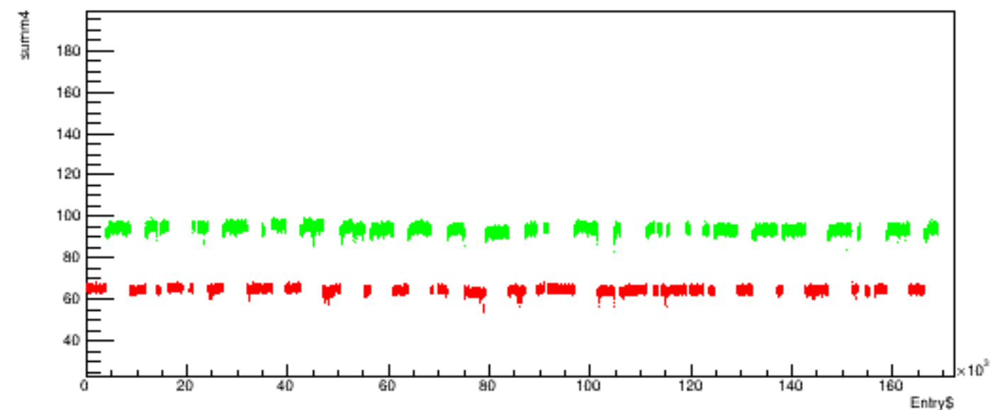
Run 4562 quartetwise, summ4 vs time
