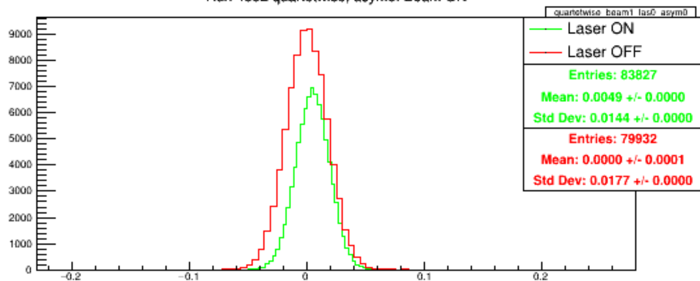
Run 4562 quartetwise, asym0: Beam ON
