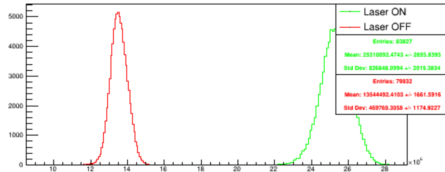
Run 4562 quartetwise, negH4: Beam ON
