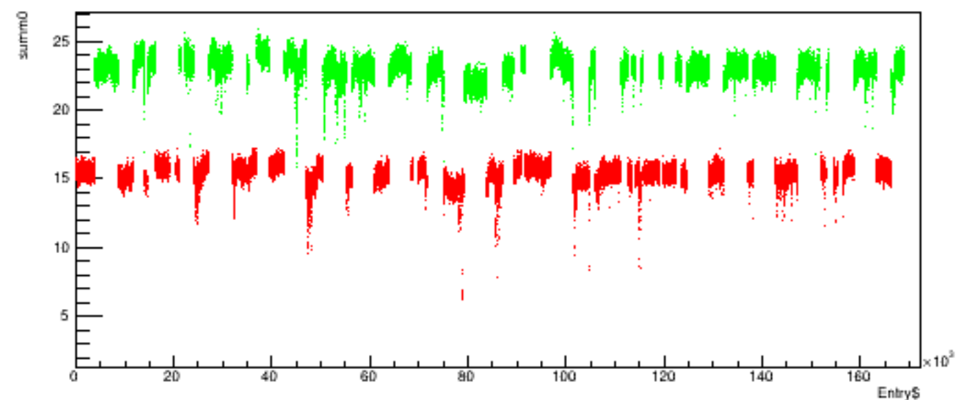
Run 4562 quartetwise, summ0 vs time
