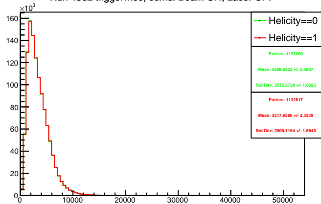
Run 4562 triggerwise, sums: Beam ON, Laser OFF
