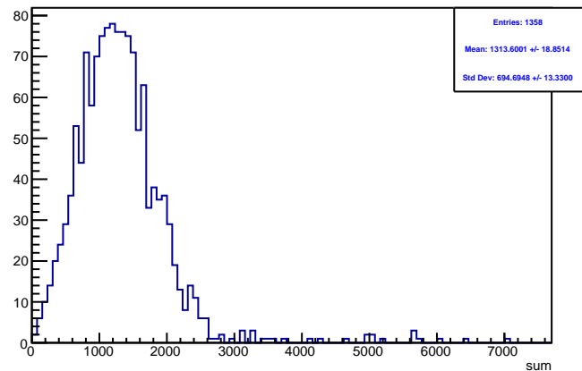
Run 4562 triggerwise, sums: Beam OFF
