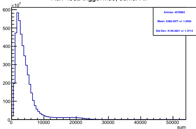
Run 4562 triggerwise, sums: All
