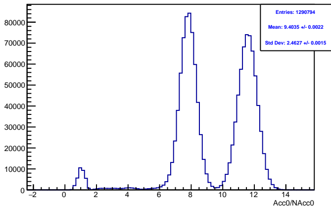
Run 4564 mpwise, acc0: Beam ON, Laser ON
