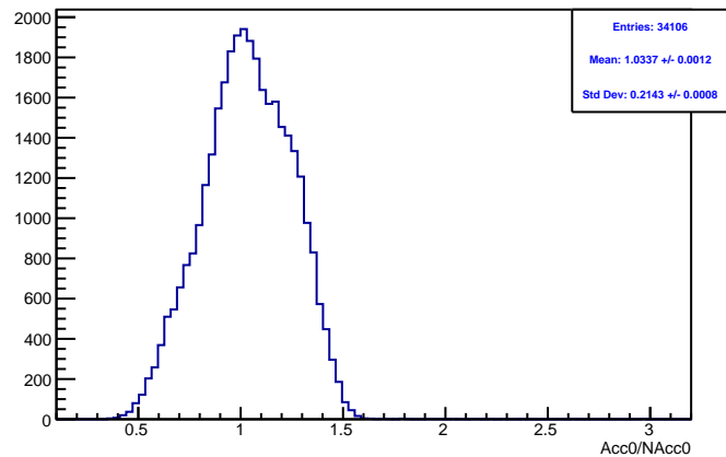
Run 4564 mpwise, acc0: Beam ON, Laser OFF
