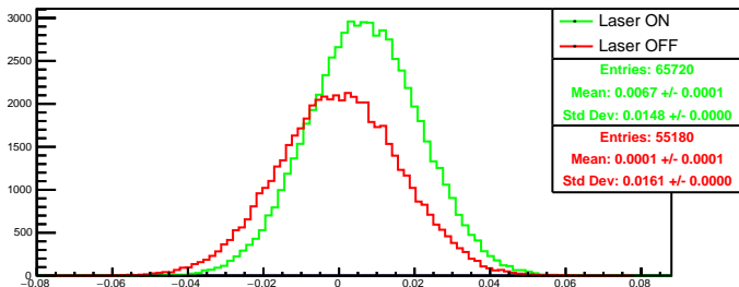
Run 4565 quartetwise, asym4: Beam ON
