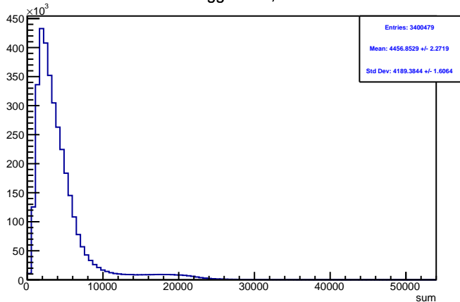
Run 4565 triggerwise, sums: All
