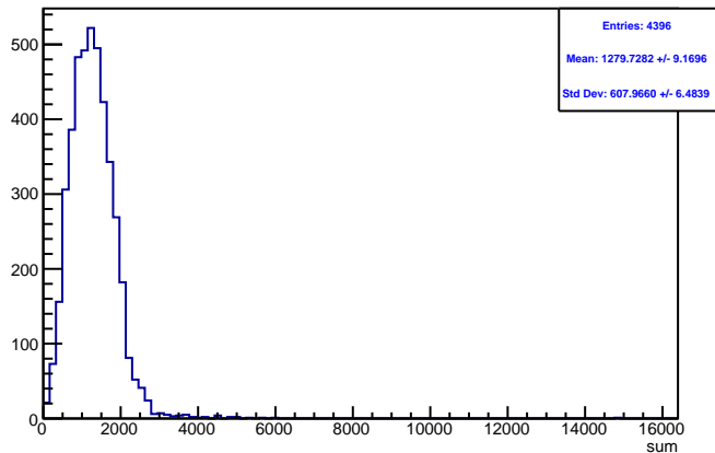
Run 4565 triggerwise, sums: Beam ON, Laser OFF
