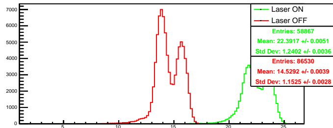
Run 4568 quartetwise, summ0: Beam ON
