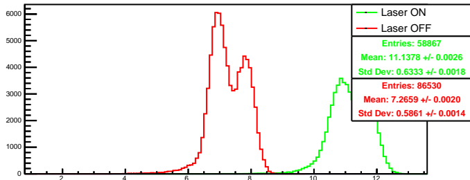
Run 4568 quartetwise, posH0: Beam ON
