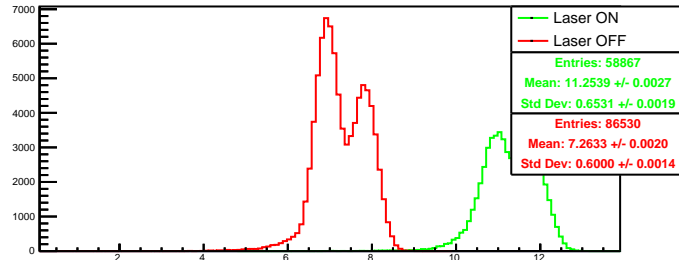
Run 4568 quartetwise, negH0: Beam ON
