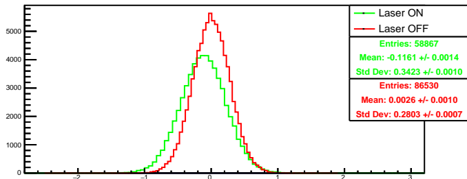
Run 4568 quartetwise, diff0: Beam ON
