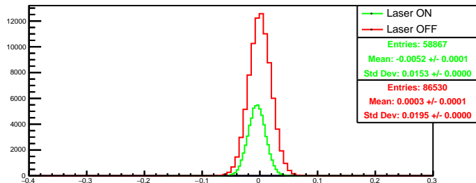
Run 4568 quartetwise, asym0: Beam ON
