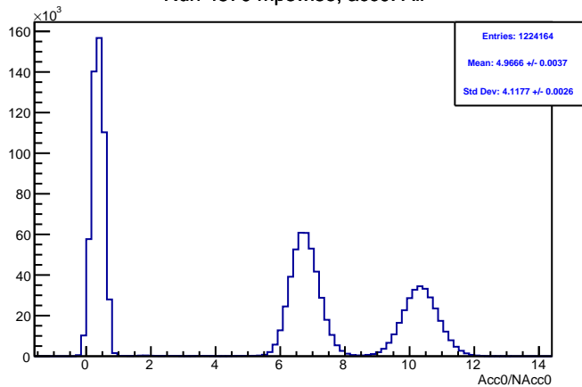
Run 4570 mpwise, acc0: All
