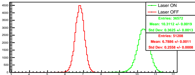
Run 4570 quartetwise, posH0: Beam ON
