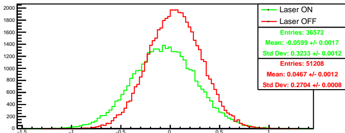
Run 4570 quartetwise, diff0: Beam ON
