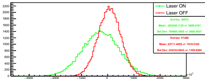
Run 4570 quartetwise, diff4: Beam ON
