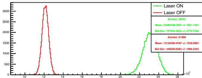
Run 4570 quartetwise, posH4: Beam ON
