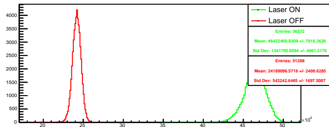
Run 4570 quartetwise, summ4: Beam ON
