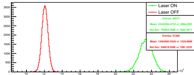
Run 4570 quartetwise, negH4: Beam ON
