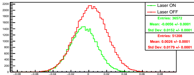
Run 4570 quartetwise, asym4: Beam ON
