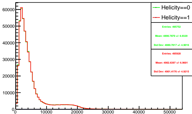
Run 4570 triggerwise, sums: Beam ON, Laser ON
