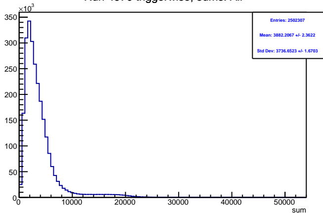
Run 4570 triggerwise, sums: All
