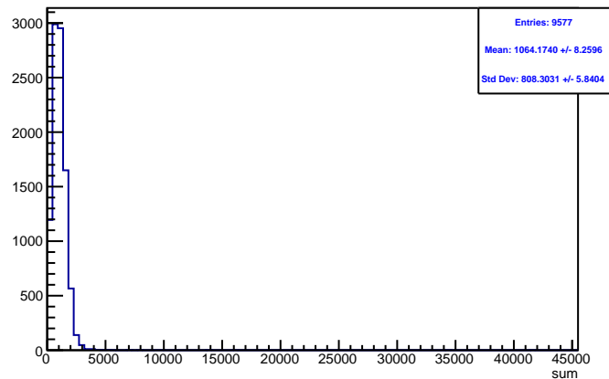
Run 4570 triggerwise, sums: Beam ON, Laser OFF
