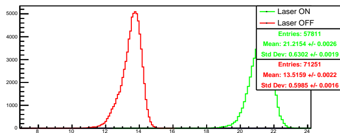
Run 4571 quartetwise, summ0: Beam ON
