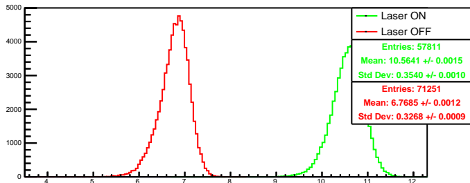
Run 4571 quartetwise, posH0: Beam ON
