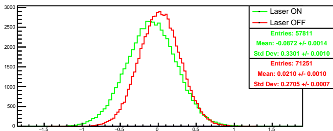
Run 4571 quartetwise, diff0: Beam ON
