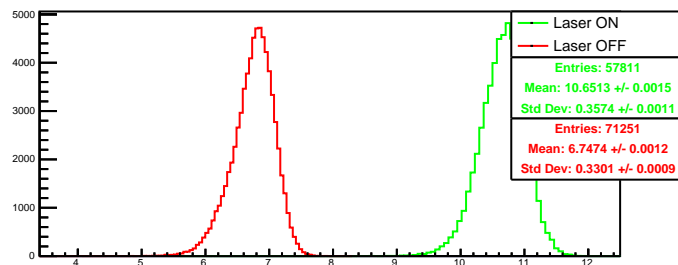
Run 4571 quartetwise, negH0: Beam ON
