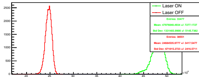
Run 4572 quartetwise, summ4: Beam ON
