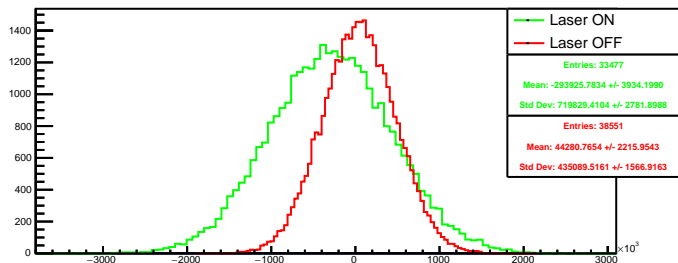
Run 4572 quartetwise, diff4: Beam ON
