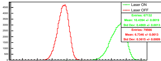
Run 4573 quartetwise, negH0: Beam ON
