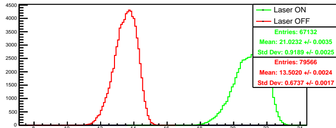
Run 4573 quartetwise, summ0: Beam ON
