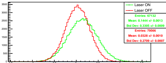
Run 4573 quartetwise, diff0: Beam ON
