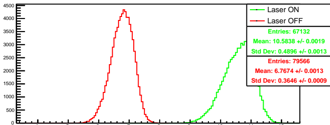
Run 4573 quartetwise, posH0: Beam ON
