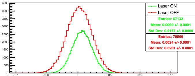
Run 4573 quartetwise, asym0: Beam ON
