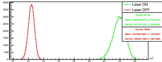
Run 4573 quartetwise, negH4: Beam ON
