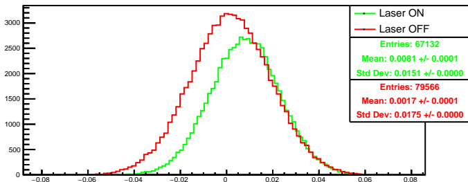
Run 4573 quartetwise, asym4: Beam ON
