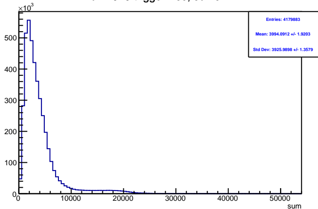
Run 4573 triggerwise, sums: All
