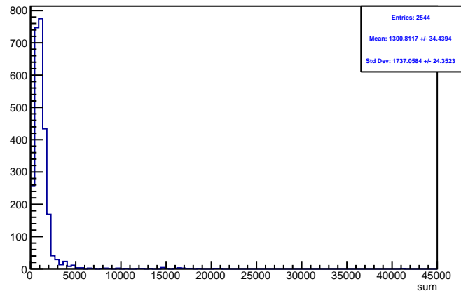
Run 4573 triggerwise, sums: Beam OFF
