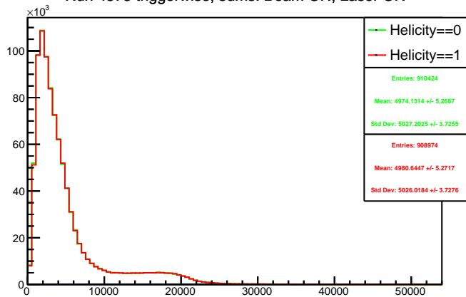
Run 4573 triggerwise, sums: Beam ON, Laser ON
