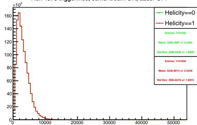
Run 4573 triggerwise, sums: Beam ON, Laser OFF
