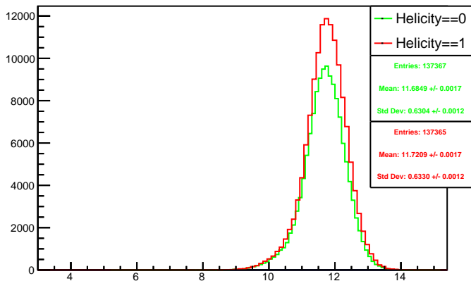
Run 4574 mpwise, acc0: Beam ON, Laser ON
