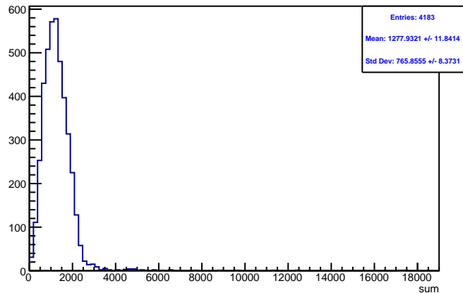
Run 4574 triggerwise, sums: Beam OFF
