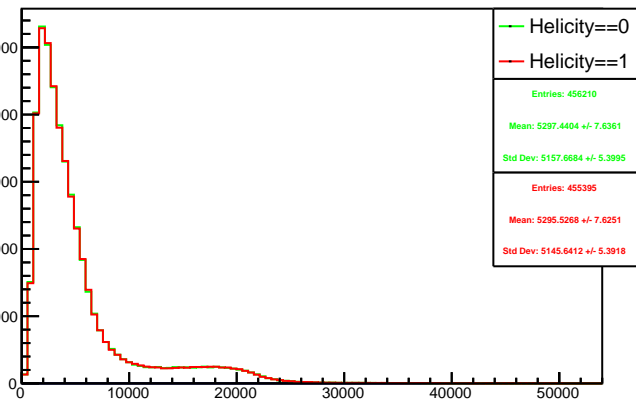
Run 4574 triggerwise, sums: Beam ON, Laser ON
