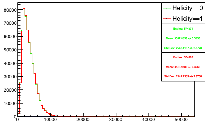
Run 4574 triggerwise, sums: Beam ON, Laser OFF
