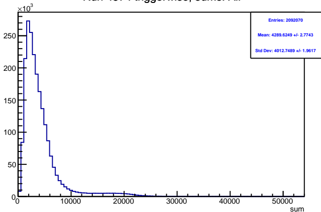
Run 4574 triggerwise, sums: All
