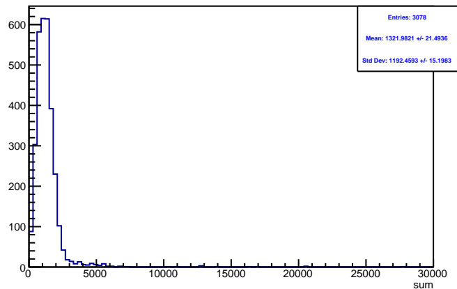
Run 4575 triggerwise, sums: Beam ON, Laser OFF
