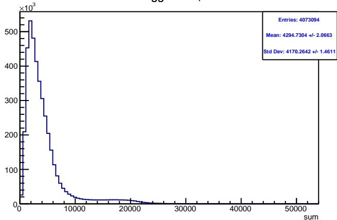
Run 4576 triggerwise, sums: All
