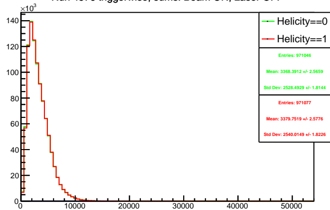
Run 4576 triggerwise, sums: Beam ON, Laser OFF
