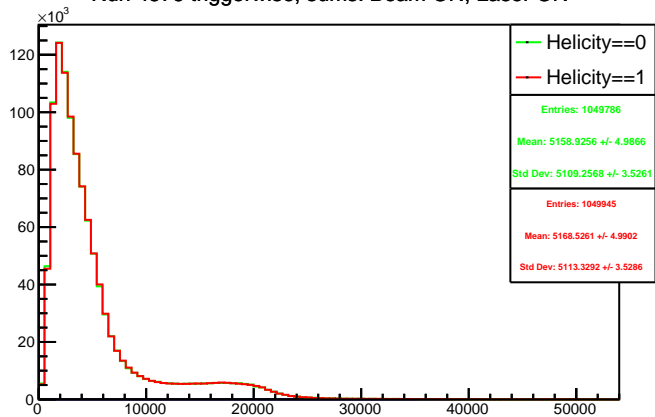
Run 4576 triggerwise, sums: Beam ON, Laser ON
