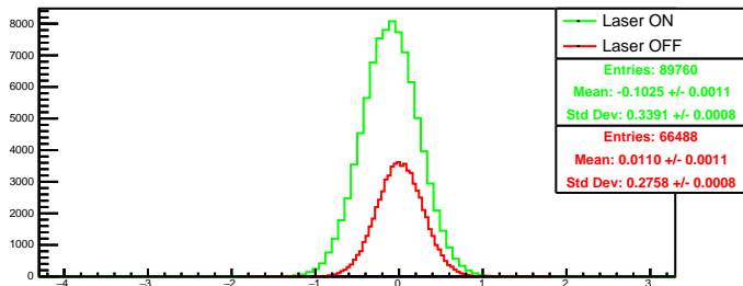
Run 4578 quartetwise, diff0: Beam ON
