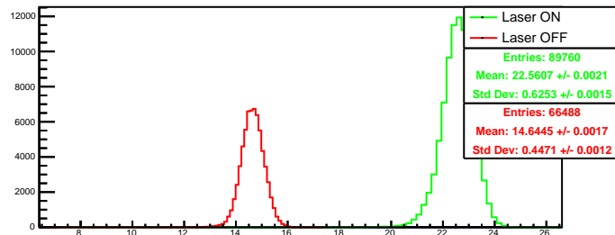
Run 4578 quartetwise, summ0: Beam ON
