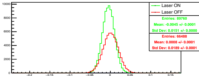
Run 4578 quartetwise, asym0: Beam ON
