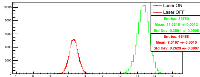
Run 4578 quartetwise, negH0: Beam ON
