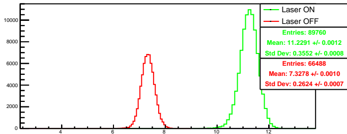
Run 4578 quartetwise, posH0: Beam ON
