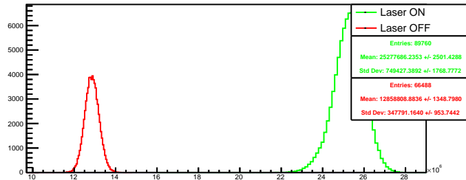
Run 4578 quartetwise, negH4: Beam ON
