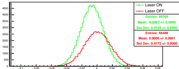
Run 4578 quartetwise, asym4: Beam ON
