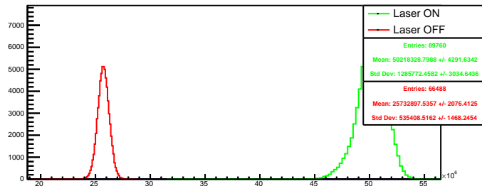
Run 4578 quartetwise, summ4: Beam ON
