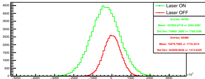
Run 4578 quartetwise, diff4: Beam ON
