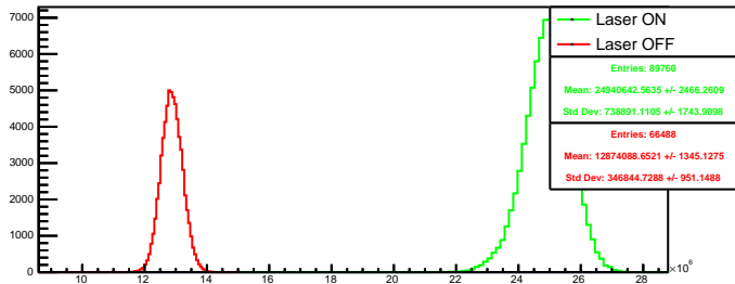
Run 4578 quartetwise, posH4: Beam ON
