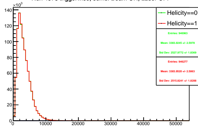
Run 4578 triggerwise, sums: Beam ON, Laser OFF
