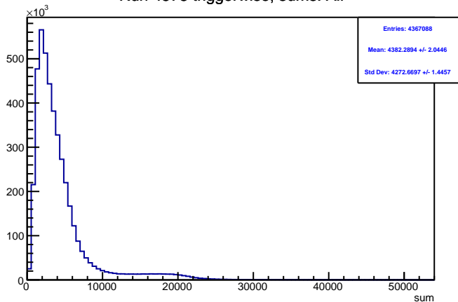
Run 4578 triggerwise, sums: All
