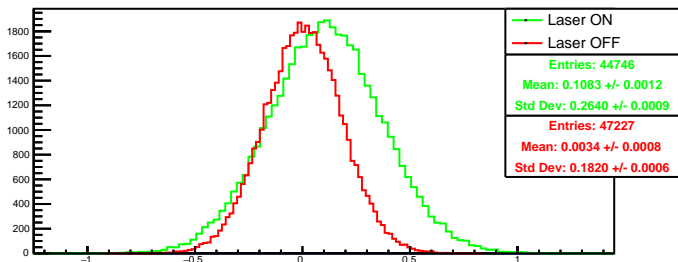
Run 4589 quartetwise, diff0: Beam ON
