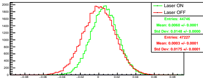
Run 4589 quartetwise, asym0: Beam ON
