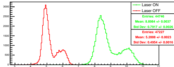
Run 4589 quartetwise, negH0: Beam ON
