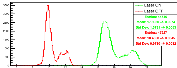
Run 4589 quartetwise, summ0: Beam ON
