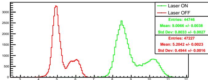
Run 4589 quartetwise, posH0: Beam ON
