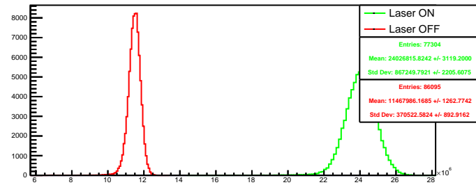
Run 4590 quartetwise, negH4: Beam ON
