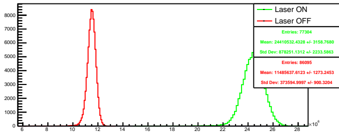
Run 4590 quartetwise, posH4: Beam ON
