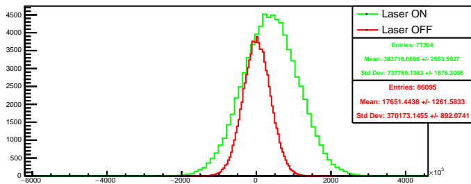
Run 4590 quartetwise, diff4: Beam ON
