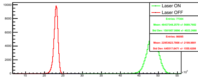
Run 4590 quartetwise, summ4: Beam ON
