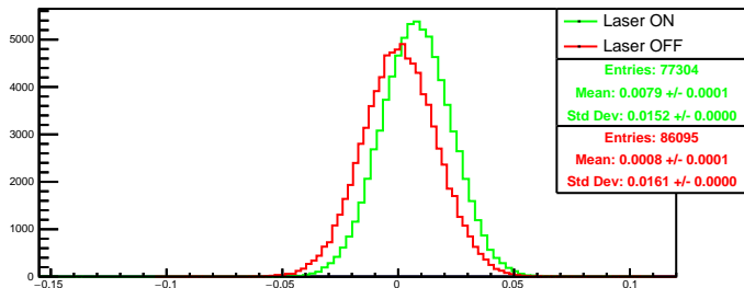
Run 4590 quartetwise, asym4: Beam ON
