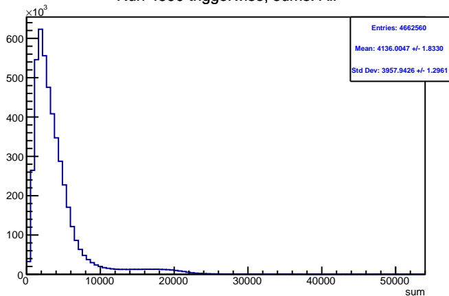
Run 4590 triggerwise, sums: All
