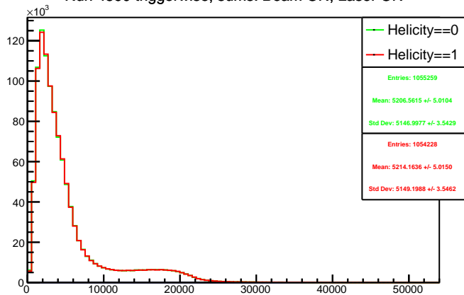
Run 4590 triggerwise, sums: Beam ON, Laser ON
