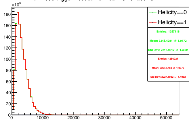
Run 4590 triggerwise, sums: Beam ON, Laser OFF
