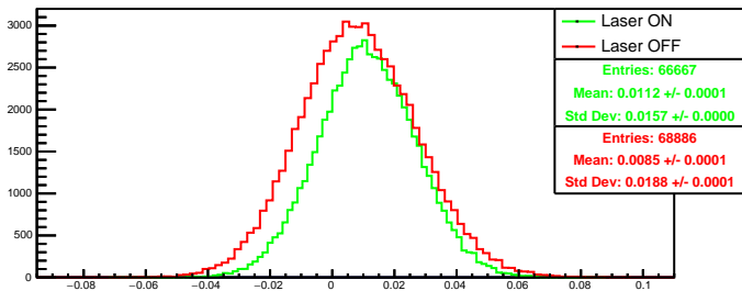
Run 4591 quartetwise, asym4: Beam ON
