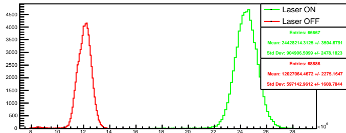
Run 4591 quartetwise, negH4: Beam ON
