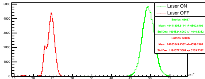
Run 4591 quartetwise, summ4: Beam ON
