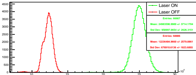
Run 4591 quartetwise, posH4: Beam ON
