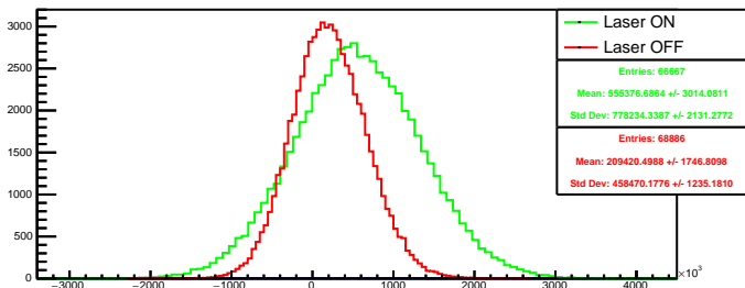
Run 4591 quartetwise, diff4: Beam ON
