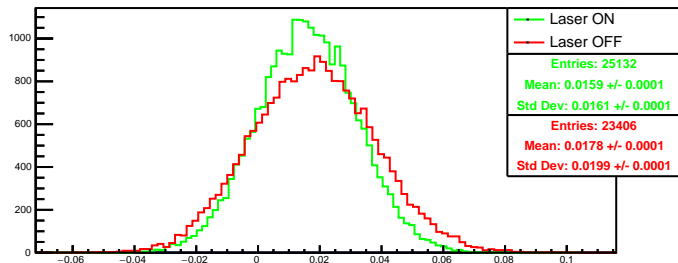
Run 4592 quartetwise, asym4: Beam ON
