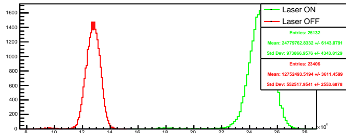
Run 4592 quartetwise, negH4: Beam ON
