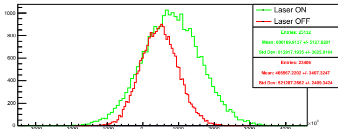
Run 4592 quartetwise, diff4: Beam ON
