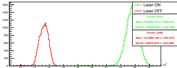
Run 4592 quartetwise, posH4: Beam ON
