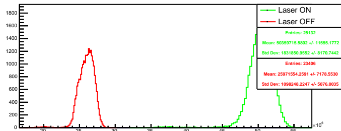
Run 4592 quartetwise, summ4: Beam ON
