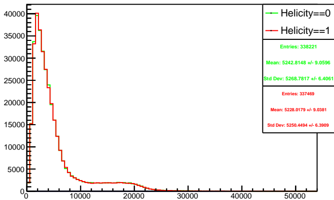
Run 4592 triggerwise, sums: Beam ON, Laser ON
