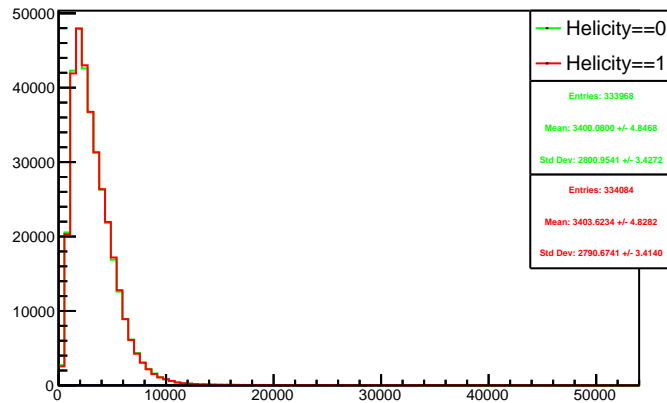
Run 4592 triggerwise, sums: Beam ON, Laser OFF
