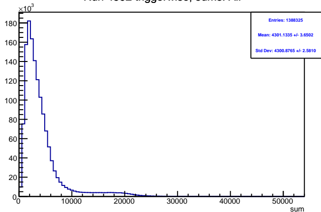
Run 4592 triggerwise, sums: All
