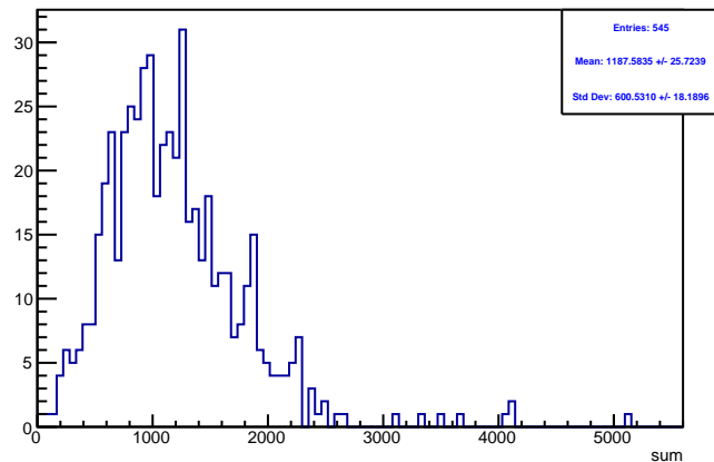
Run 4592 triggerwise, sums: Beam ON, Laser OFF
