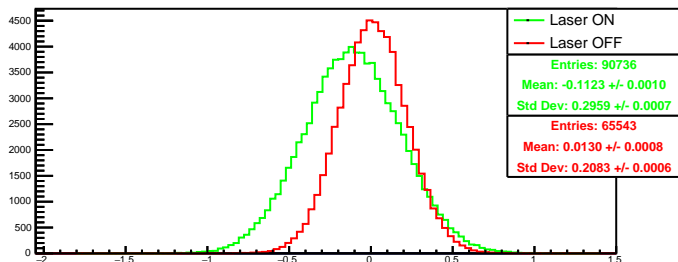
Run 4594 quartetwise, diff0: Beam ON
