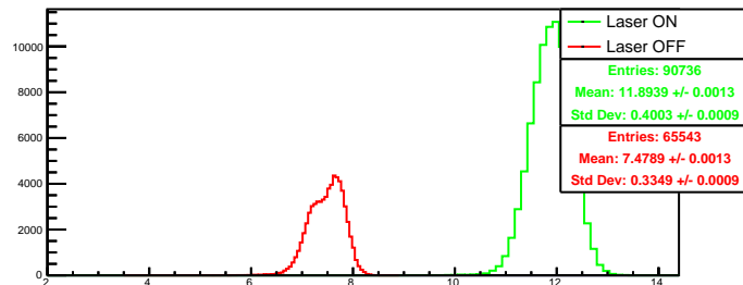
Run 4594 quartetwise, negH0: Beam ON
