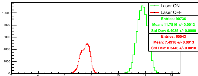
Run 4594 quartetwise, posH0: Beam ON
