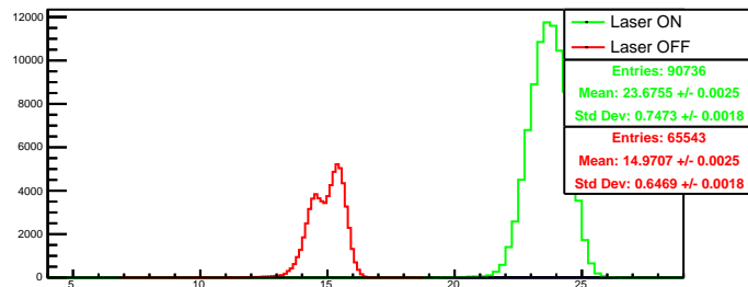
Run 4594 quartetwise, summ0: Beam ON
