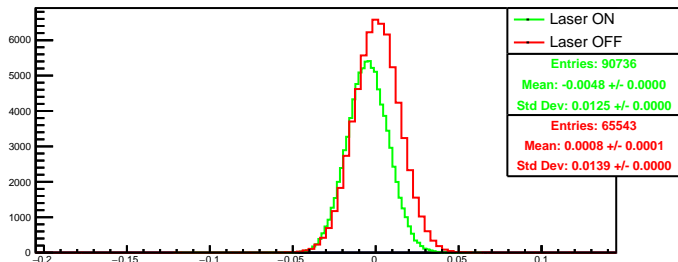
Run 4594 quartetwise, asym0: Beam ON
