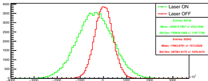
Run 4594 quartetwise, diff4: Beam ON
