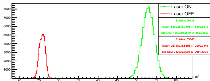
Run 4594 quartetwise, summ4: Beam ON
