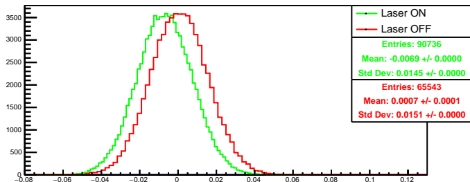
Run 4594 quartetwise, asym4: Beam ON
