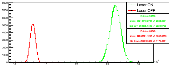
Run 4594 quartetwise, posH4: Beam ON
