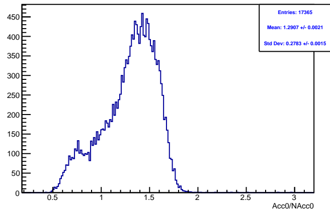
Run 4595 mpwise, acc0: Beam ON, Laser OFF
