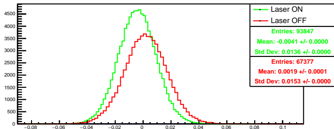
Run 4595 quartetwise, asym0: Beam ON
