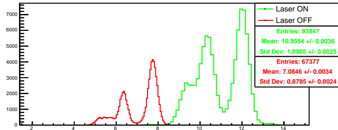
Run 4595 quartetwise, negH0: Beam ON
