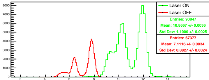
Run 4595 quartetwise, posH0: Beam ON
