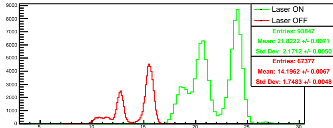
Run 4595 quartetwise, summ0: Beam ON
