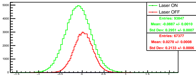
Run 4595 quartetwise, diff0: Beam ON
